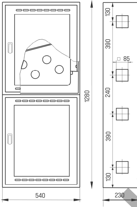
Fig. 4 - Fire Cabinet PRESTIGE wall-mounted
