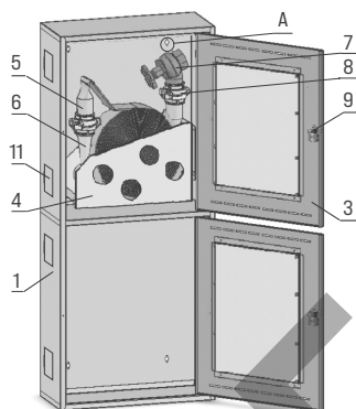
Fig.1 - Fire Hose Cabinet Complete Set PRESTIGE 03-W
